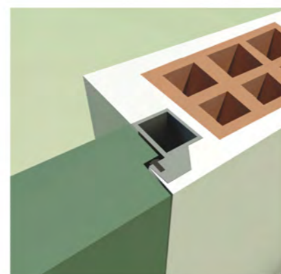
Porta filomuro lato esterno, apertura a spingere Flush to wall door with outside push opening
